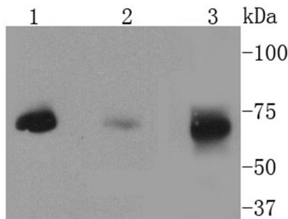
Fig. 1. Western blot analysis of MEKK2 on different lysates using anti-MEKK2 antibody at 1/1,000 dilution. Positive control: Lane 1: HepG2; Lane 2: Rat brain; Lane 3: SW480
